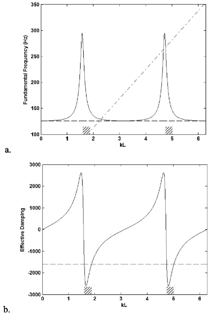
FIG. 11. (a) Fundamental frequency of vocal fold vibration and (b) corresponding effective damping induced by the subglottal system as a function of the product of wave number and tracheal length for an open-ended and lossless trachea tube. —: solution curve; - - -: (a) natural frequency of the vocal folds and (b) critical effective damping at which the equality in Eq. (A11) is reached; - · - : f = (c/2\pi L) \cdot kL for L = 100 cm; shaded area: regions possible for phonation onset.
